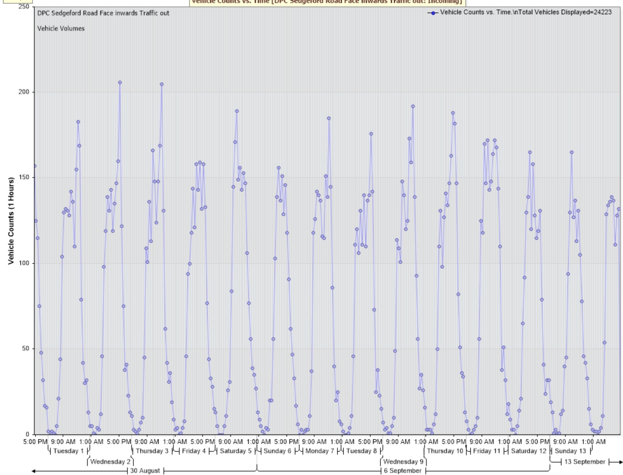
Vehicle Counts vs. Time [DPC Sedgford Road Face inwards Traffic out: Incoming]
