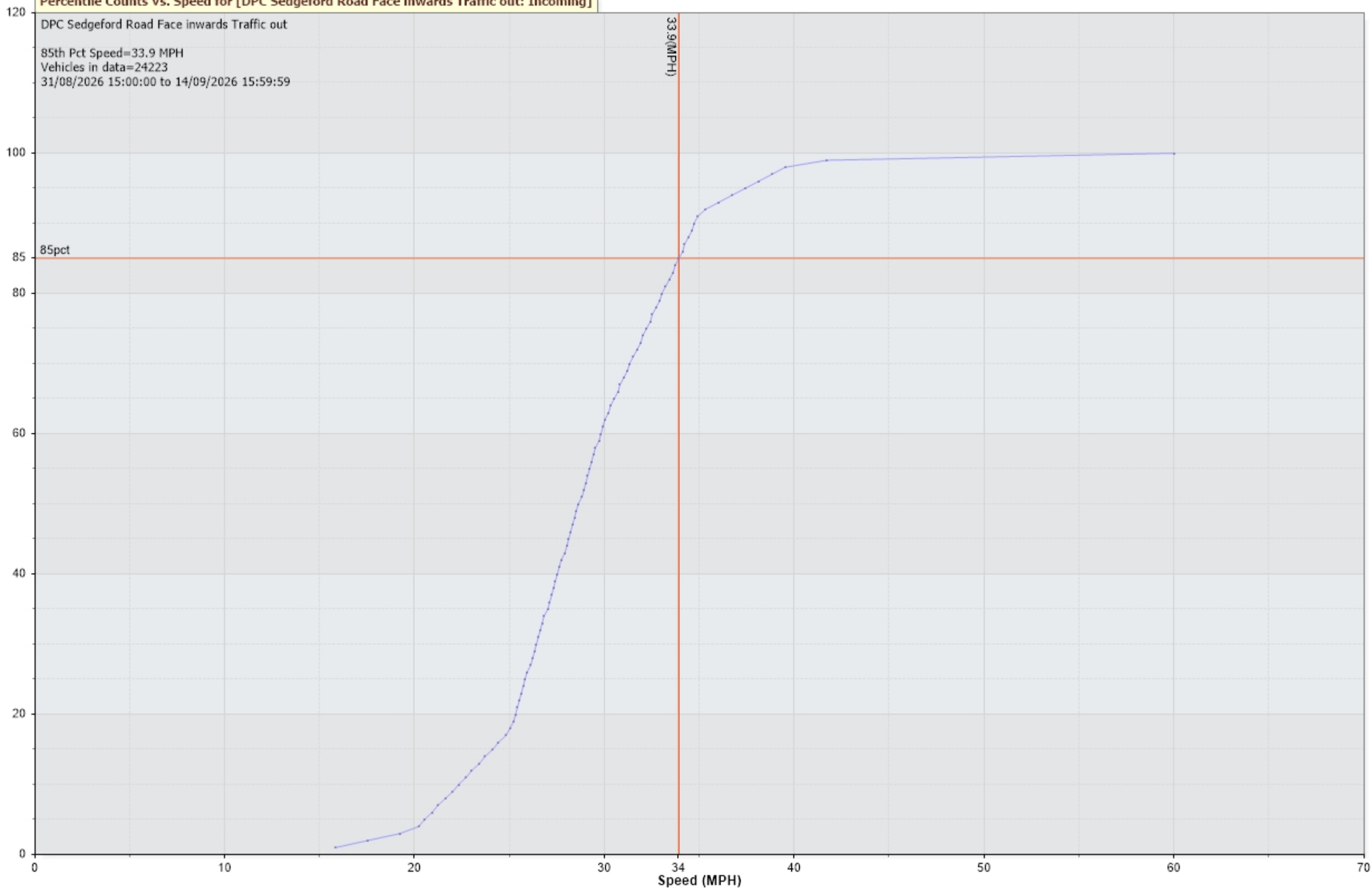
Percentile Counts Vs. Speed for [DPC Sedgeford Road Face inwards Traffic out: Incoming]
