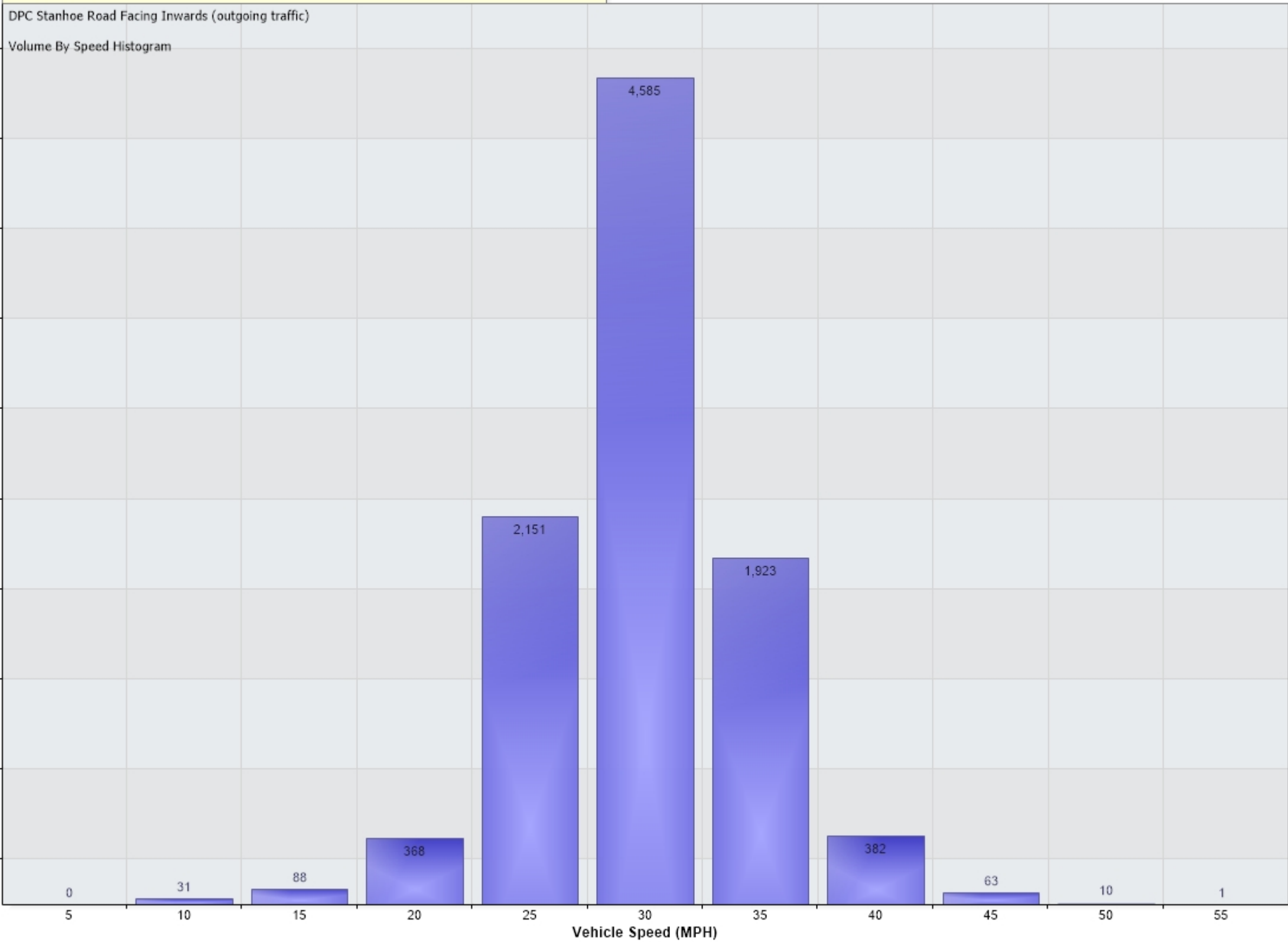
Vehicle Counts Vs. Speed [DPC Stanhoe Road Facing Inwards (outgoing traffic): Incoming]
